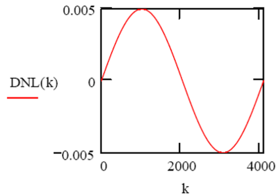
Figure 2: DNL of a 12-bit ADC.
